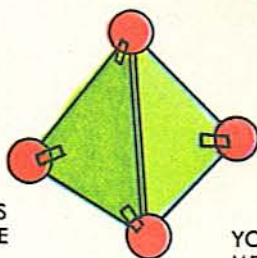
TWO LABORATORY MODELS SHOWING THE METHANE MOLECULE.
